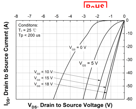
Figure 14. 3rd Quadrant Characteristic at T_J = 25\text{ }^\circ\text{C}
